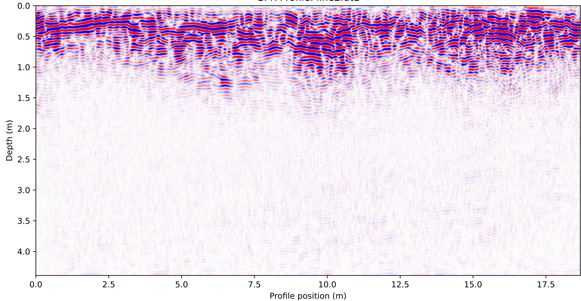
GPR Profile: line2.dt1
